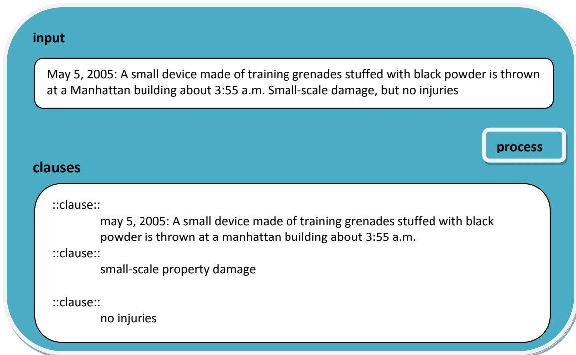
Figure 3: clause-breaking module
